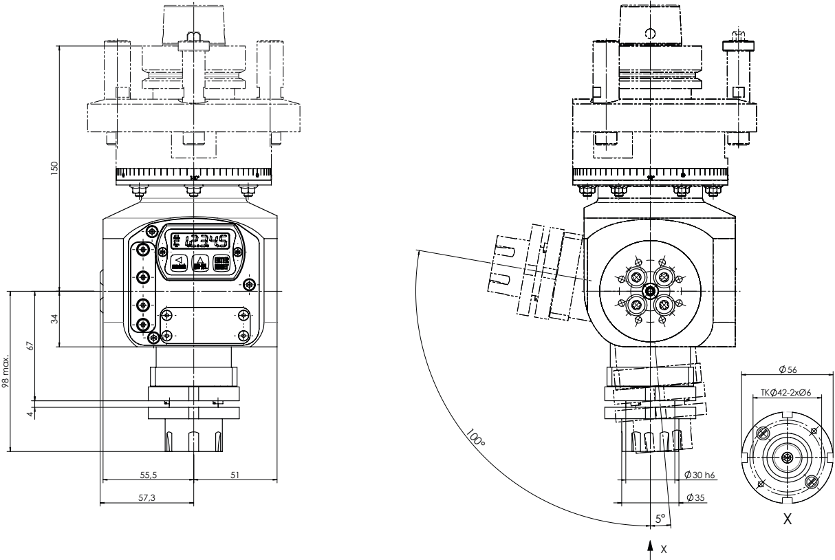
HSK - F63 HOMAG / WEEKE / WEINMANN
