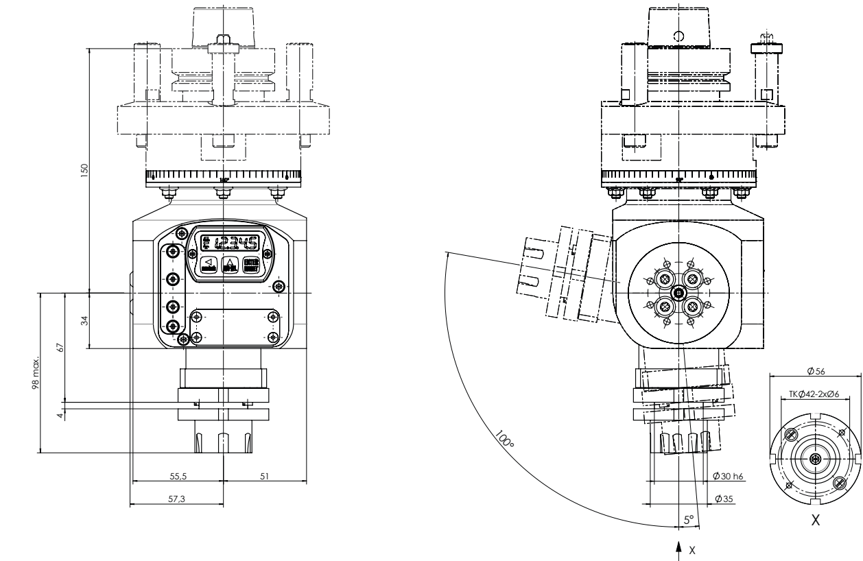
HSK - F63 HOMAG / WEEKE / WEINMANN
