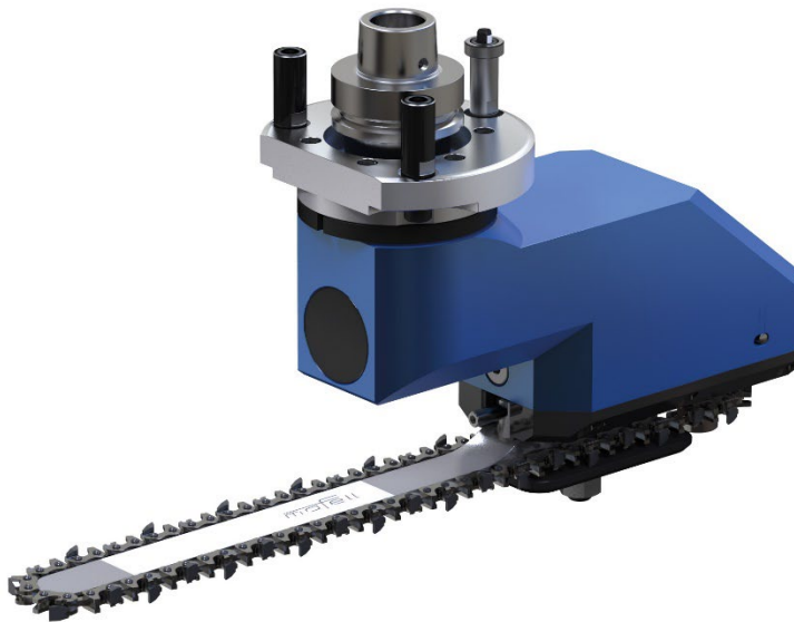
Image 3: Completely new machining options with improved CATENO F mortising chain unit
