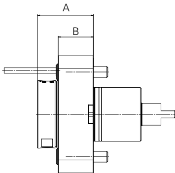
BENZ Solidfix® / Collet chuck
